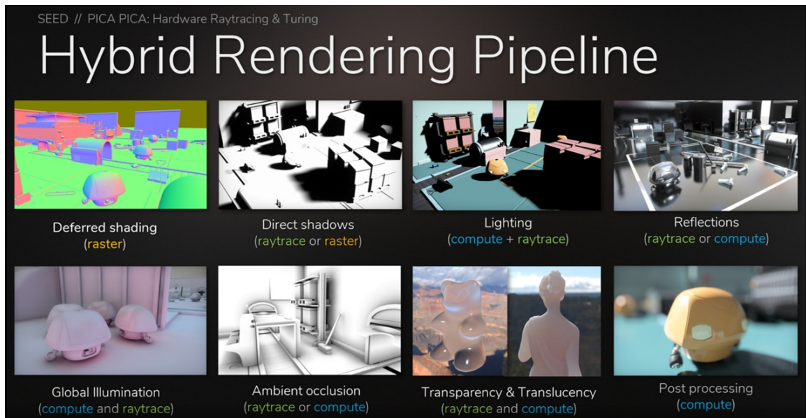
Figure 16. Hybrid Rendering Pipeline
